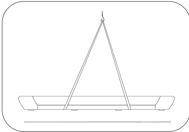
Fig. 1 – Crane install – strap locations
