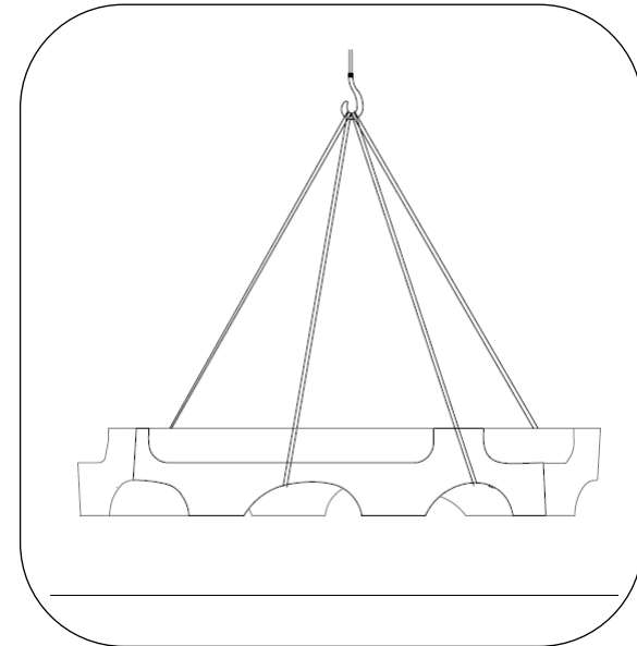
Fig. 1 – Crane install – strap locations
