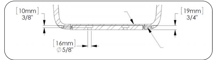
Fig. 1 – surface mount base section
