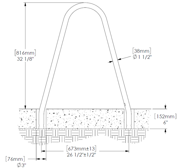
Side Elevation, showing core drill sizes
